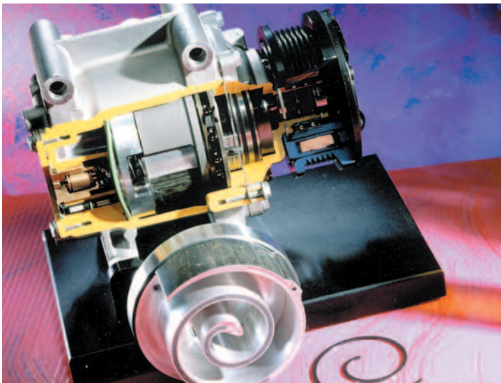
The VICTREX PEEK polymer seals are located on the tips of the fixed and orbiting scrolls.
