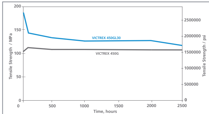
Figure 2: Retention of Tensile Strength After Conditioning in Steam at 200°C (392°F) and 1.4MPa (200psi)
