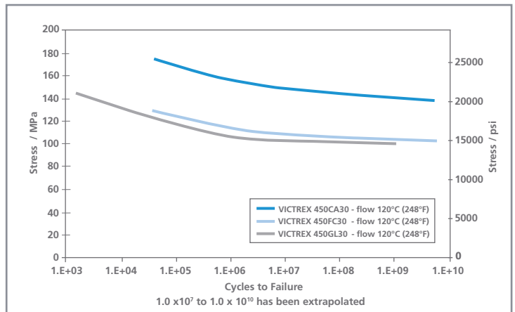
Figure 3: VICTREX PEEK Polymer Flexural Fatigue Endurance
