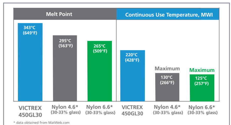
Figure 1: Temperature Comparison of VICTREX 450GL30 vs 30% Glass Reinforced Nylon
