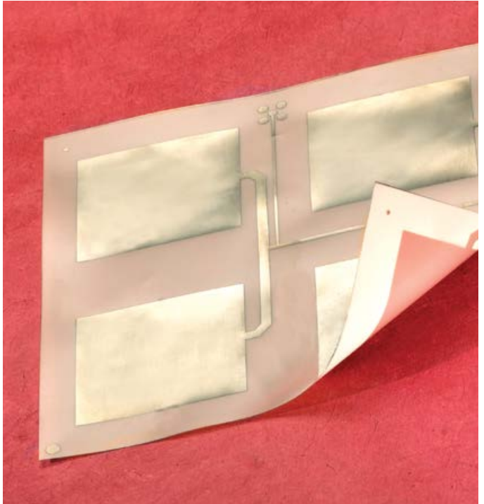
Clean, dry and contaminant free substrates are important prerequisites in the thermoplastic metallisation process.
